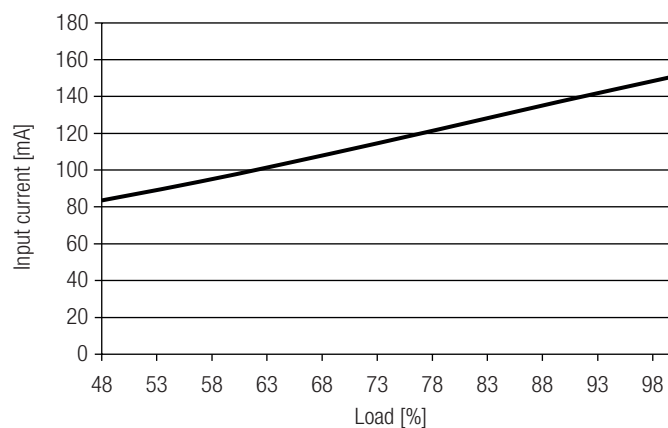
Input current vs load
