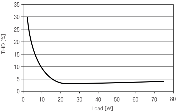
4.5 THD vs. Load
