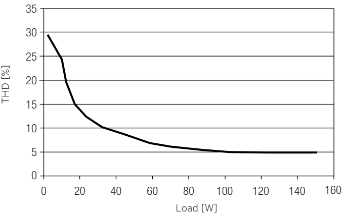
4.5 THD vs. Load
