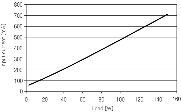
4.4 Input current vs. Load
